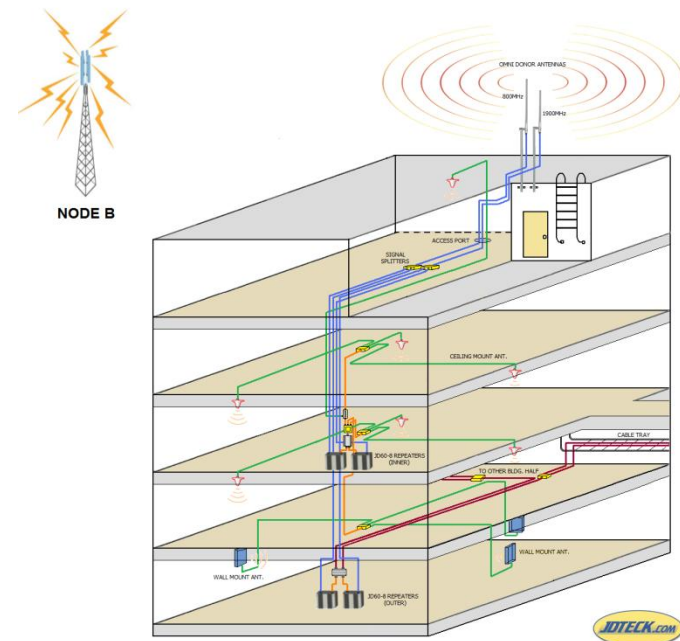
Figure 1 shows the application of the cellular repeaters.
